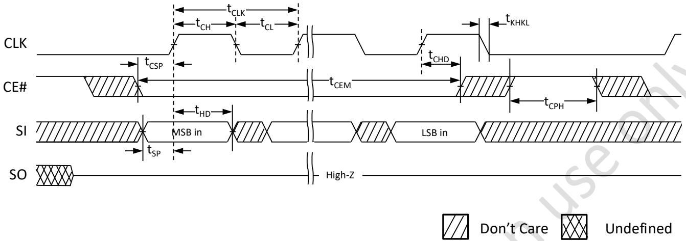
Figure 20: Input Timing
