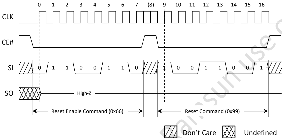
Figure 17 : SPI Reset
